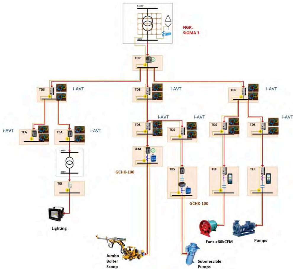
Figure1: I-Gard Technology installed in a Mining Operation
